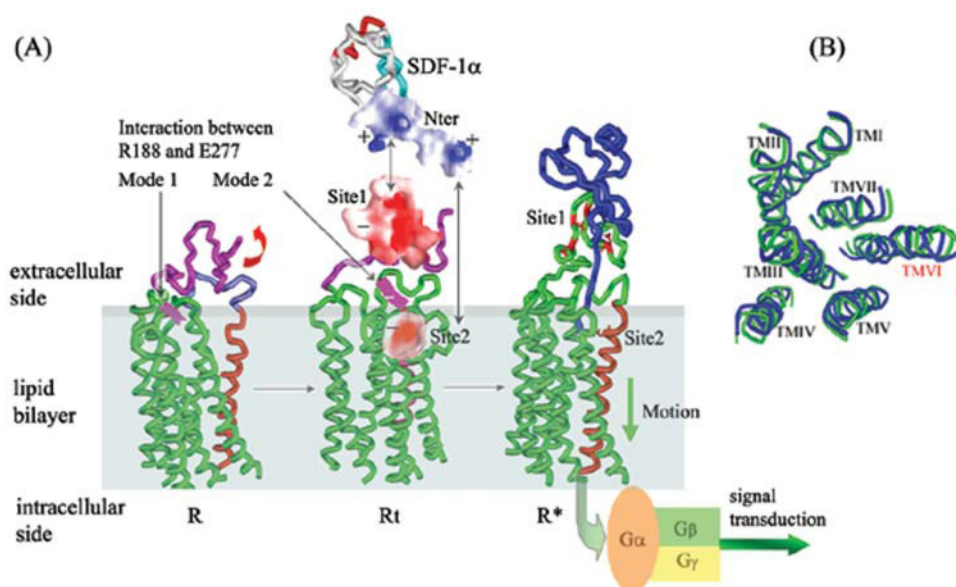
FIGURE 7 Overall conformational transitions in the process of CXCR4 binding with SDF-1 \alpha . (A) CXCR4 changes from its lowest-energy conformation ( R ) to transition state ( Rt ). Interaction between the Arg188-Glu277 salt bridge changes from Mode I to Mode II at same time. After recognition of conserved negative-charged cluster (— symbol, in red, Site1 represented as molecular surface; the range of the color panel is the same as that in Fig. 4) at Nter of CXCR4 with positive-charged cluster (+ symbol, molecular surface indicated in blue) at Nter of SDF-1 \alpha (shown as black arrow); conformational changes of ED-CXCR4 results in exposure of Site 2 in TMs domain. Thereafter, when SDF-1 \alpha —CXCR4 complex is formed, the receptor comes to its active state ( R* ). (B) Top view of conformation comparison for R (in green) with R* (in blue). TM VI has more significant conformational change while the whole RMSD of C \alpha of TMs is 0.95.
