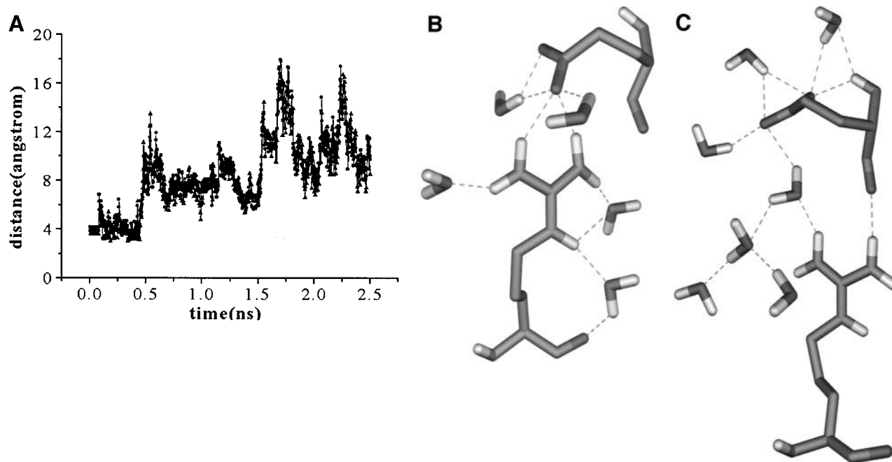
FIGURE 5 (A) Distance fluctuations for atoms (C \zeta , N \eta^1 , and N \eta^2 of Arg188; C \delta of Glu277) of the Arg188-Glu277 salt bridge. ■: Distance from C \zeta Arg188 to C \delta Glu277; ●: distance from N \eta^1 Arg188 to C \delta Glu277; and ▲: distance from N \eta^2 Arg188 to C \delta Glu277. (B) and (C) Typical interaction modes (B, Mode I; C, Mode II) of Arg188-Glu277 pair including relative water molecules.
